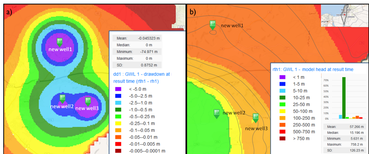
Figure 2: a) Recalculated drawdown by the THEIS well function and b) groundwater level simulated by the MODFLOW model combined with the analytical calculation.
